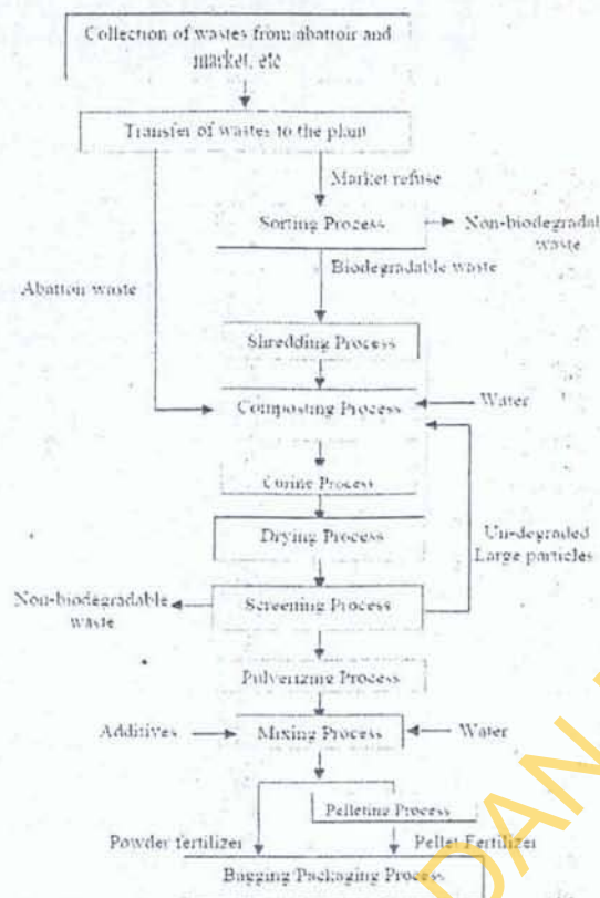
Fig. 1: Flow chart of the organic fertilizer processing operations
