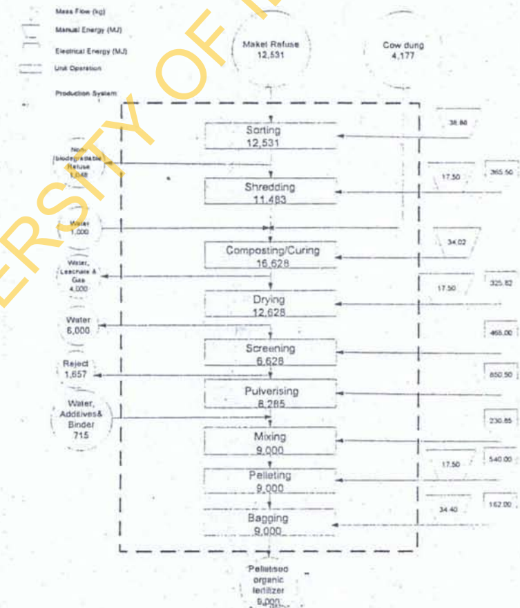
Fig.3: Energy and mass flow diagram for the production of pelletised organic fertilizer
