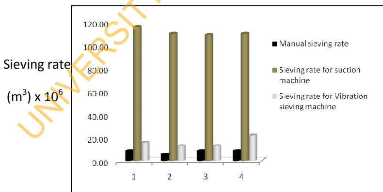
Figure 5 Sieving Rates for Manual and Mechanical processes
