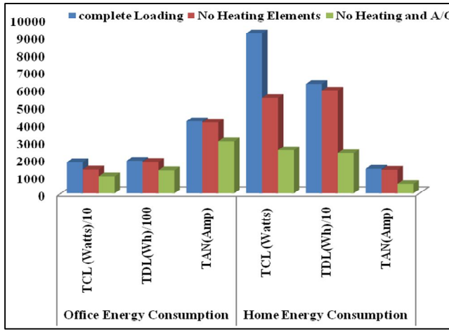
Fig. 3. Comparison of AC sizing results ( T_{CL} , T_{DL} , T_{AN} ) for different selected loadings
