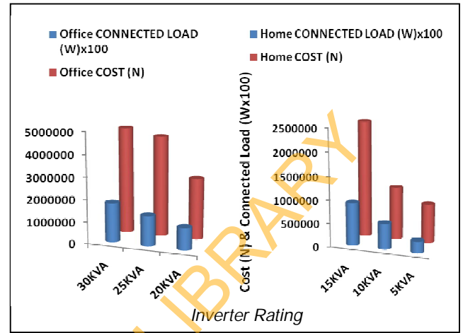
Fig. 6. Energy-cost variations for Inverters units
