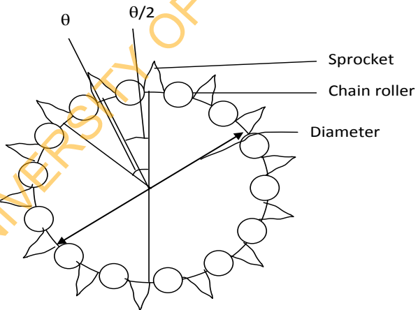
Figure 4: Type of sprocket used in chain drive
