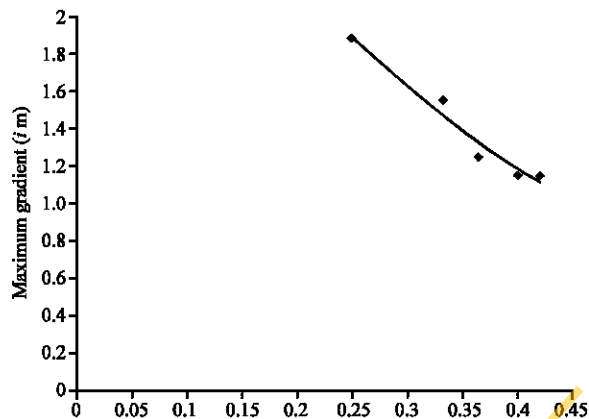
Fig. 1: Graph of maximum gradient ( i_m ) against porosity
