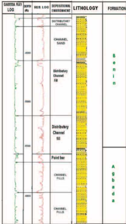
Figure 21a. Gamma ray and Resistivity Logs showing depositional environments from depth interval between 4000 ft (1363.63 m) to 6500 ft (1969.69 m) within well BLG1.
