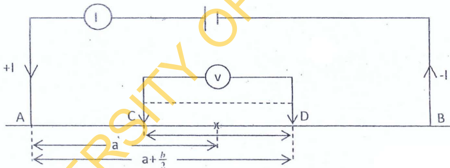
Fig.3: Schlumberger configuration.
