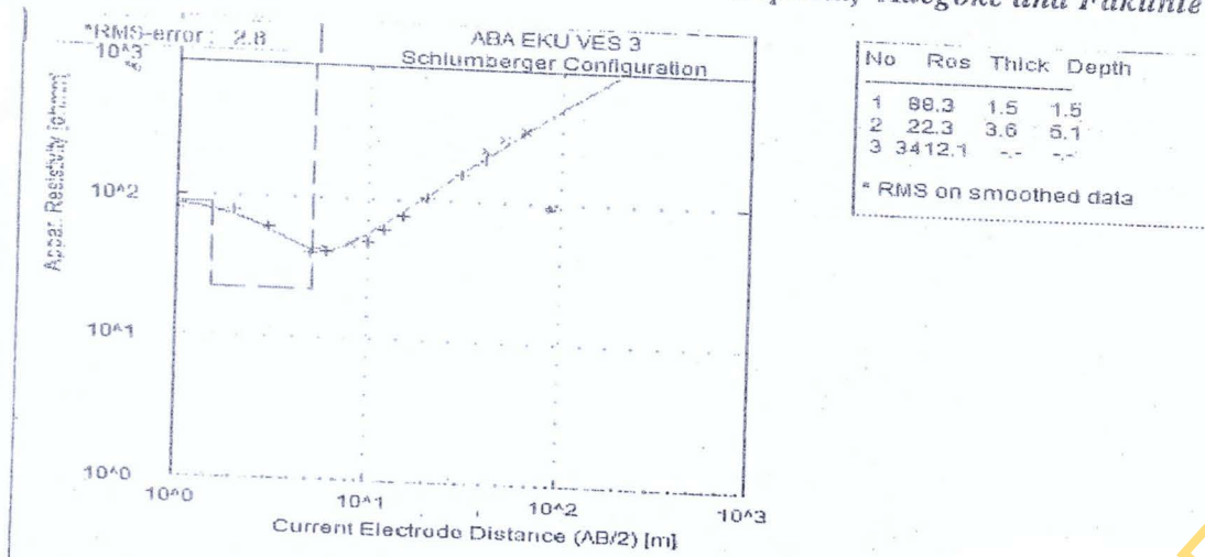
Fig.4: Layer model Interpretation of VES point of side A of Aba- Eku dump site
