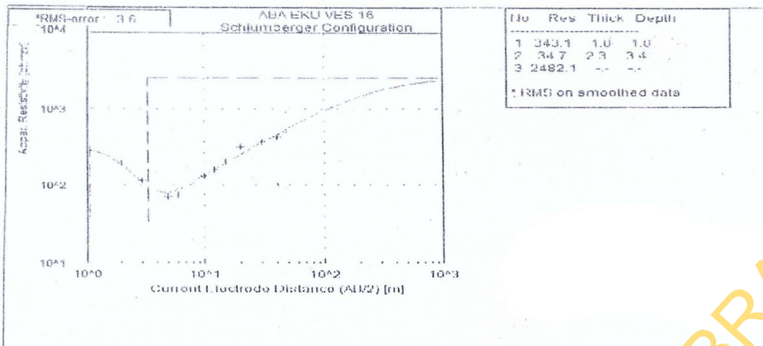
Fig.7: Layer model interpretation of VES point of side D of Aba- Eku Dump site
