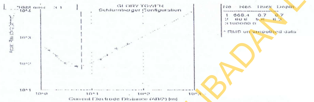
Fig.8: Layer model interpretation of VES point of Glory Tower Schools control point to Aba Eku dump site.
