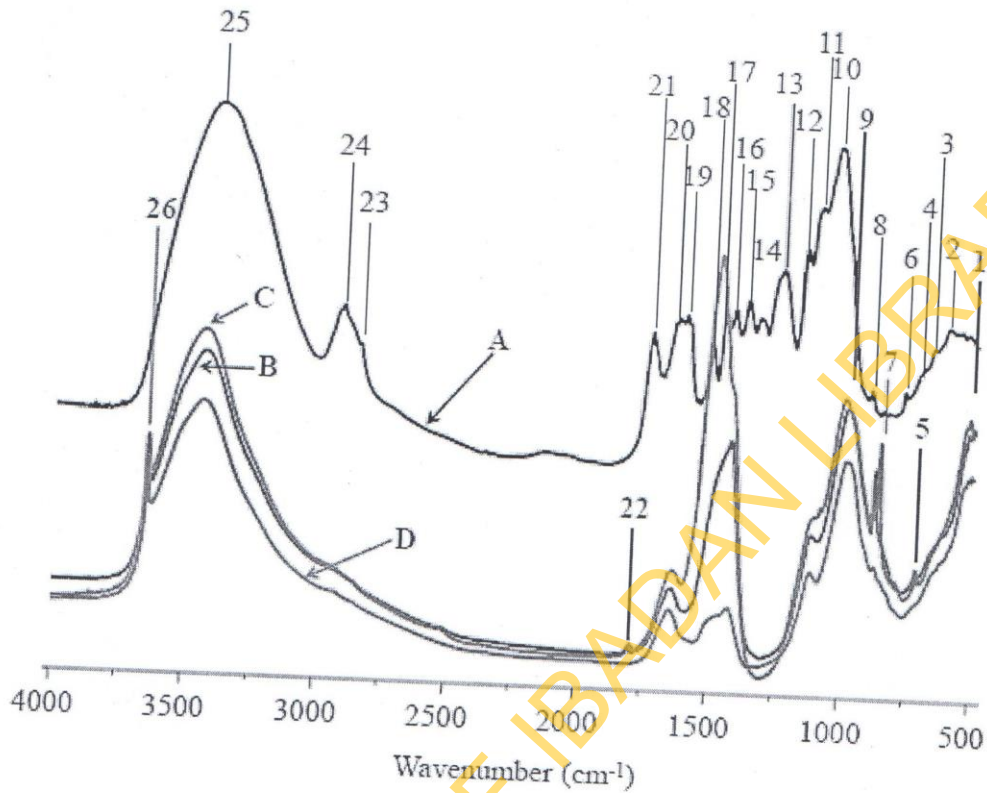
Figure 2 - FTIR spectra of (A) Laccosperma secundiflorum , (B) L. secundiflorum /cement mix, (C) L. secundiflorum /cement/ \text{CaCl}_2 , and (D) L. secundiflorum /cement/30 min cold water extraction. Each spectrum is an average of spectra from two specimens. Peak position and assignment as well as structural polymer for each peak are presented in Table 4.
