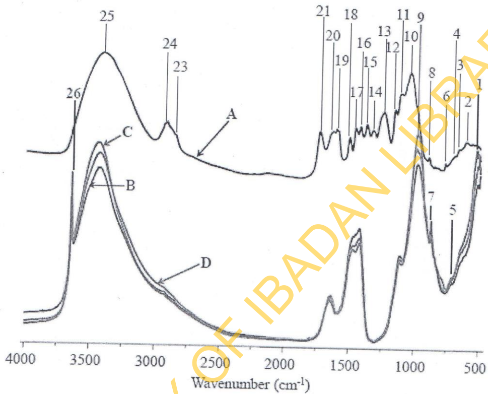
Figure 1 - FTIR spectra of (A) Eremospatha macrocarpa , (B) E. macrocarpa /cement mix, (C) E. macrocarpa /cement/ \text{CaCl}_2 , and (D) E. macrocarpa /cement/30 min cold water extraction. Each spectrum is an average of spectra from two specimens. Peak position and assignment as well as structural polymer for each peak are presented in Table 3.
