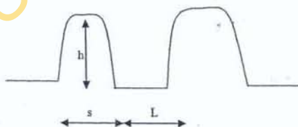
Fig 1. Conical-shaped road bump
