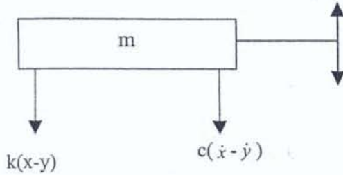
Fig 3. Free-body diagram of the road bump-vehicle interaction
