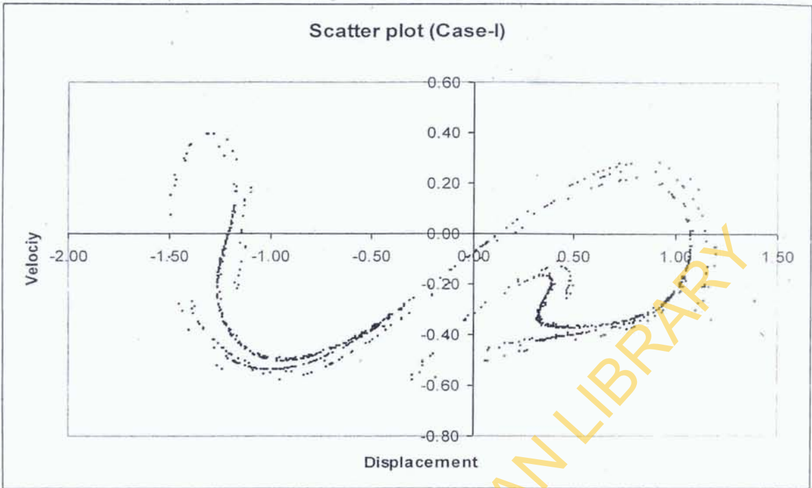
Figure 5: Steady scatter plot (Case-I) phase variables on phase plane computed at the end of 70 th excitation period
