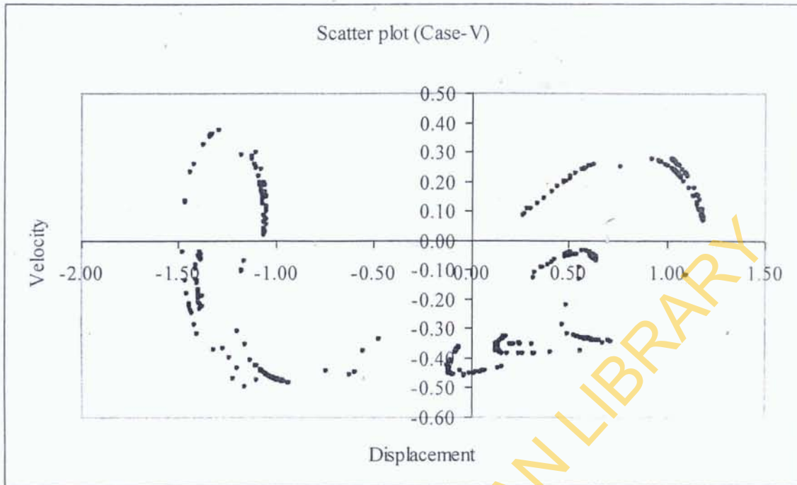
Figure 9: Steady scatter plot (Case-V) phase variables on phase plane computed at the end of 70 th excitation period
