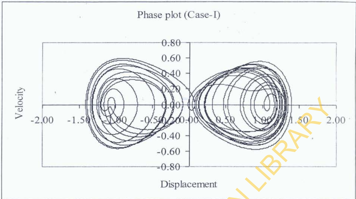
Figure 1: Steady Phase plot (Case-I) computed by V500 over 41 st to 70 th excitation period
