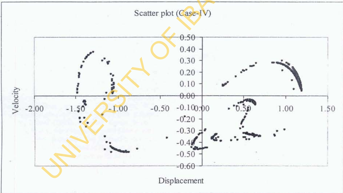
Figure 8: Steady scatter plot (Case-IV) phase variables on phase plane computed at the end of 70 th excitation period
