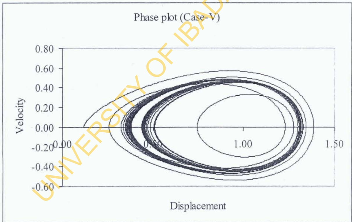
Figure 2: Steady Phase plot (Case-V) computed by V500 over 41 st to 70 th excitation period
