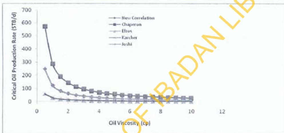
Figure 3. Influence of oil viscosity on critical rate.
