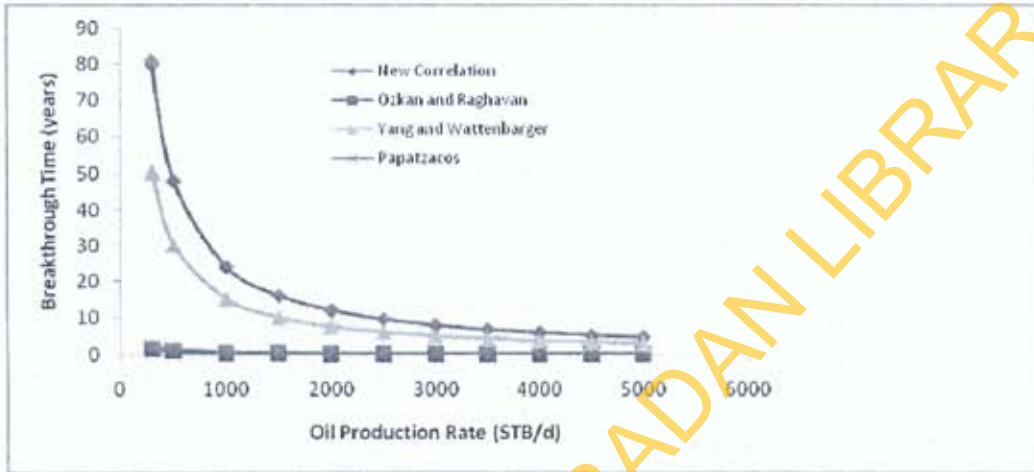
Figure 5. Influence of oil production rate on breakthrough time.
