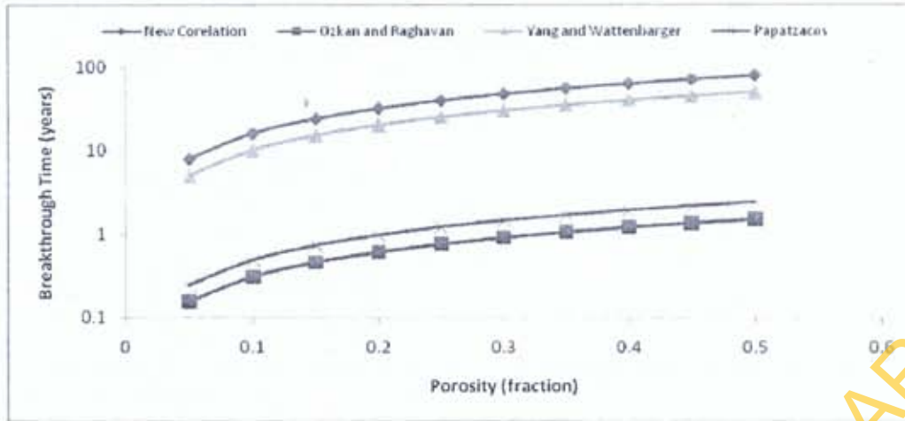
Figure 7. Influence of formation porosity on breakthrough time.
