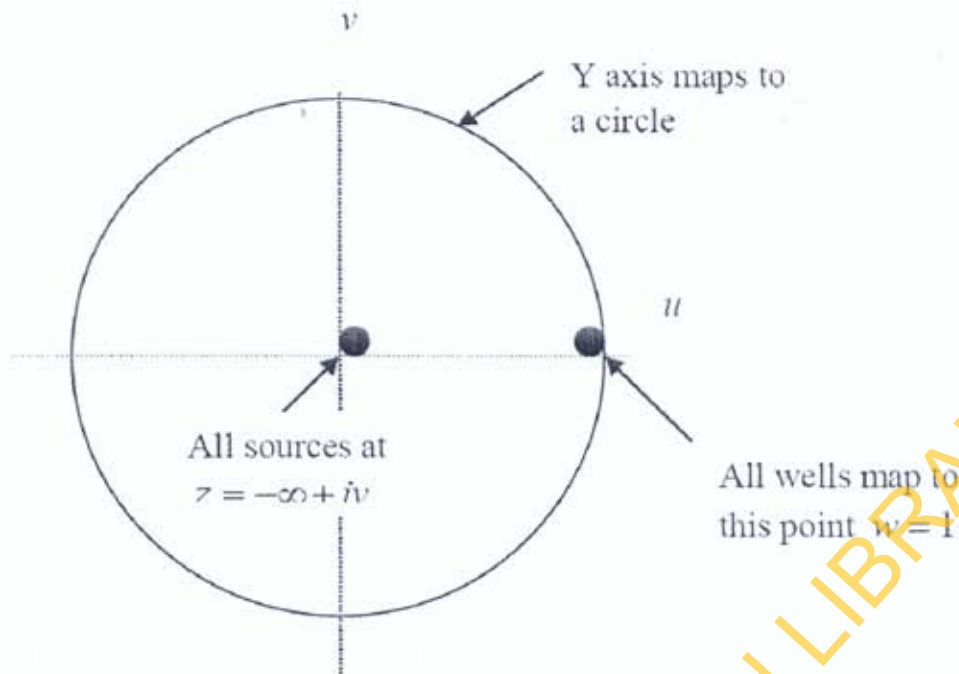
Figure A2. Conformal Map of Reservoir using w = u + iv = e^{(2\pi z/h)} .
