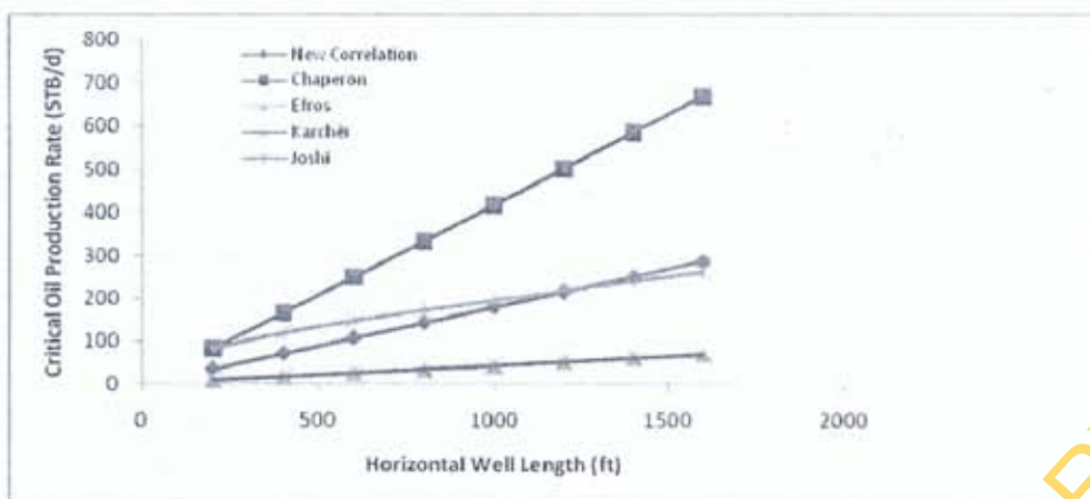
Figure 2. Influence of oil horizontal well length on critical rate.
