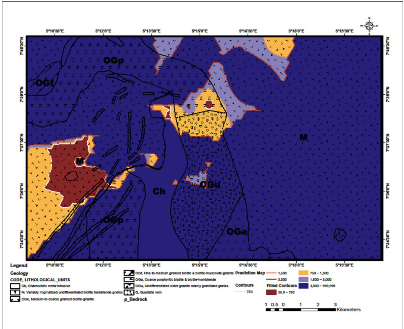
Figure 5.24: Overburden Thickness Classification Map
