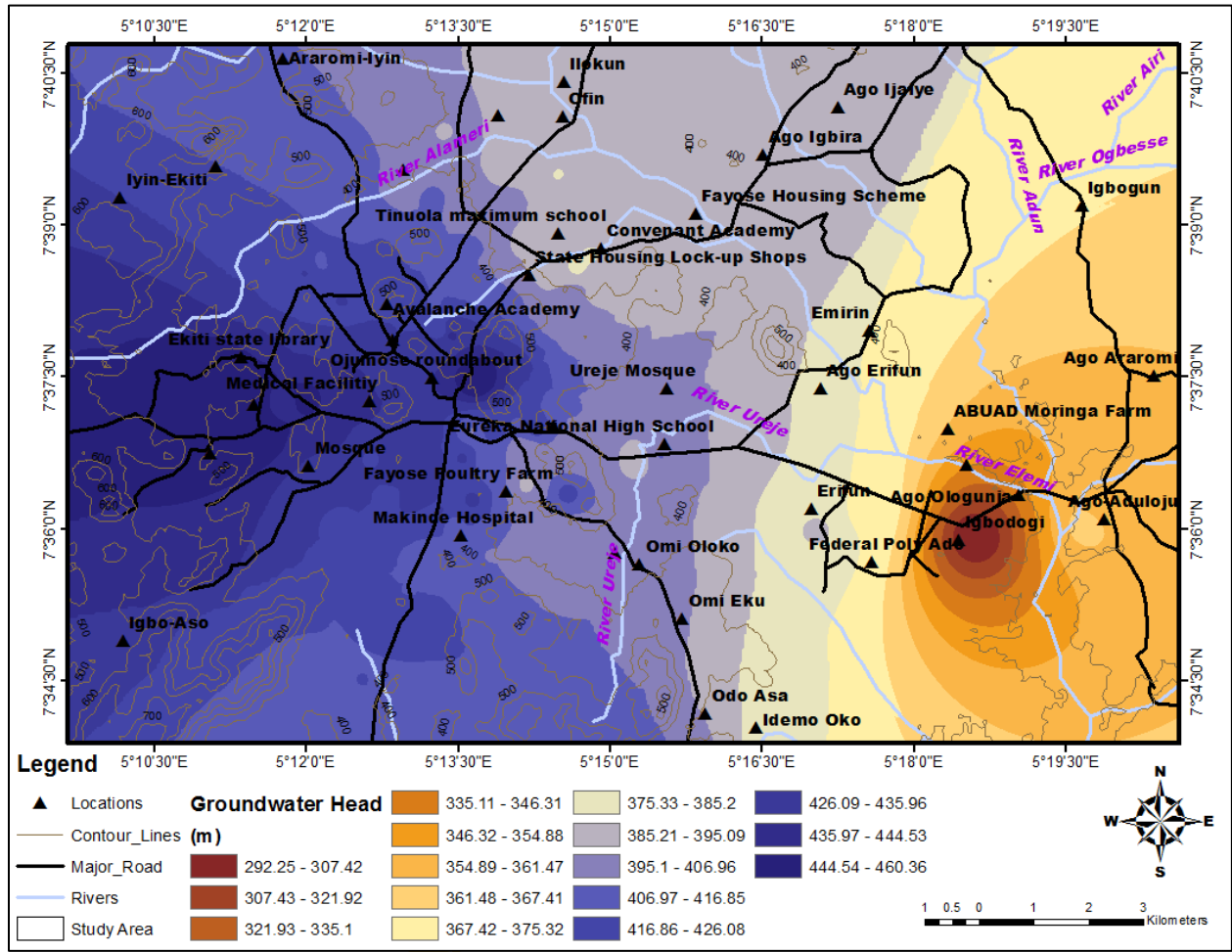
Figure 5.37: Groundwater head map
