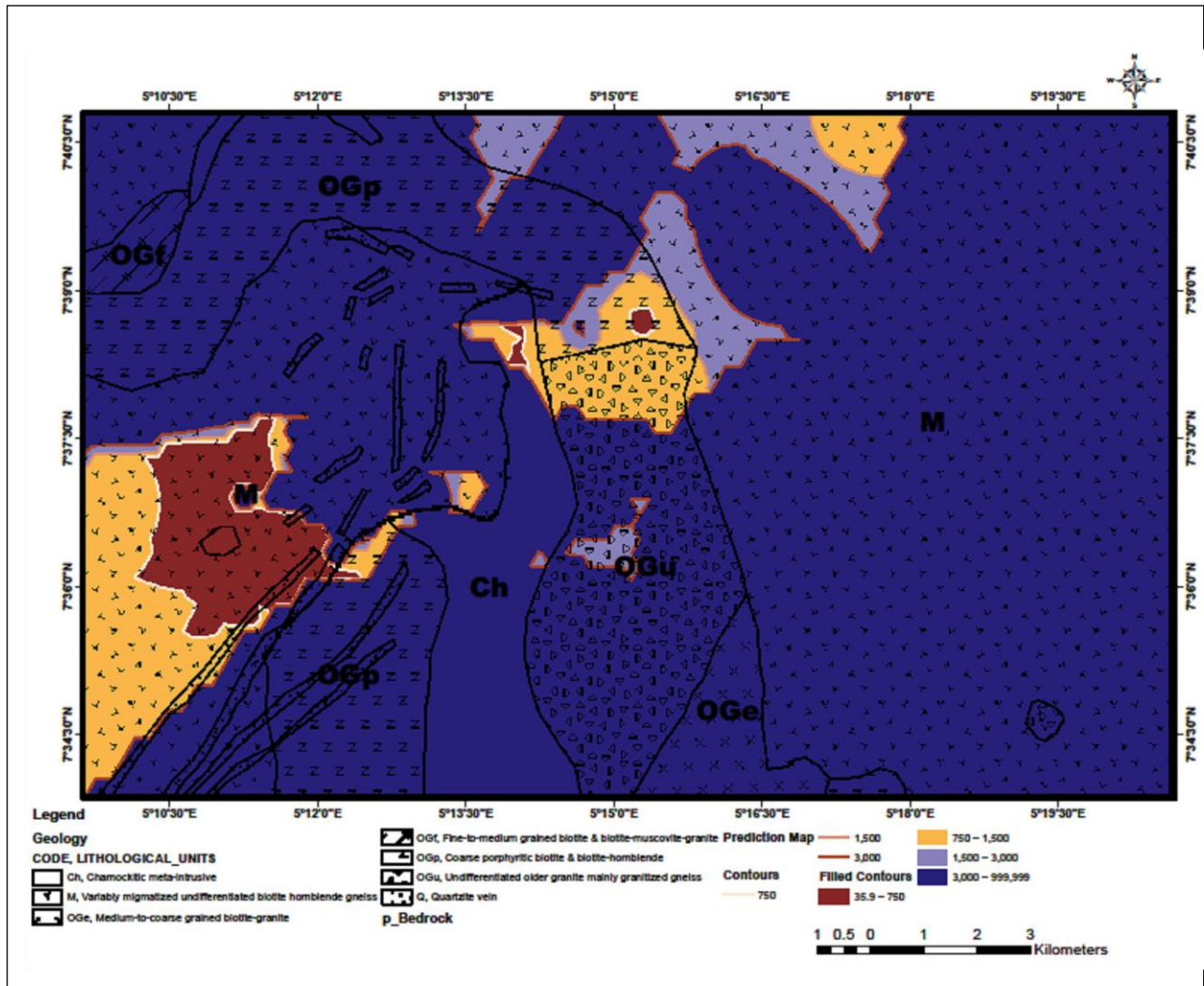
Figure 5.21: Bedrock Resistivity Classification Map
