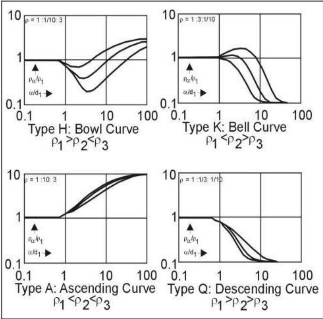
Figure 2.3: Four types of three-layer VES curves (Adapted from Resistivity Methods: Environmental Geophysics US EPA.htm)
