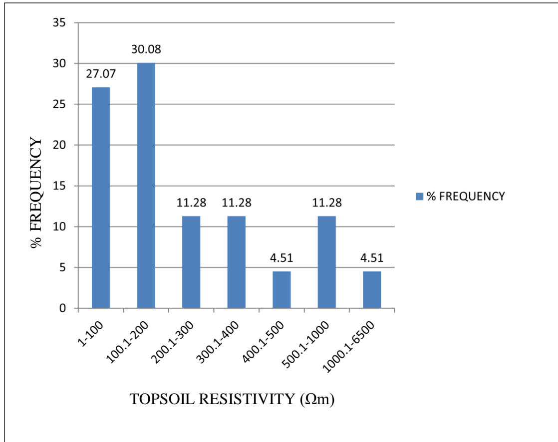
Figure 5.7: Frequency Distribution of Topsoil Resistivity
