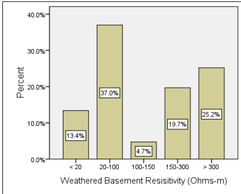
Figure 5.17: Weathered Basement Resistivity Classification of Ado-Ekiti
