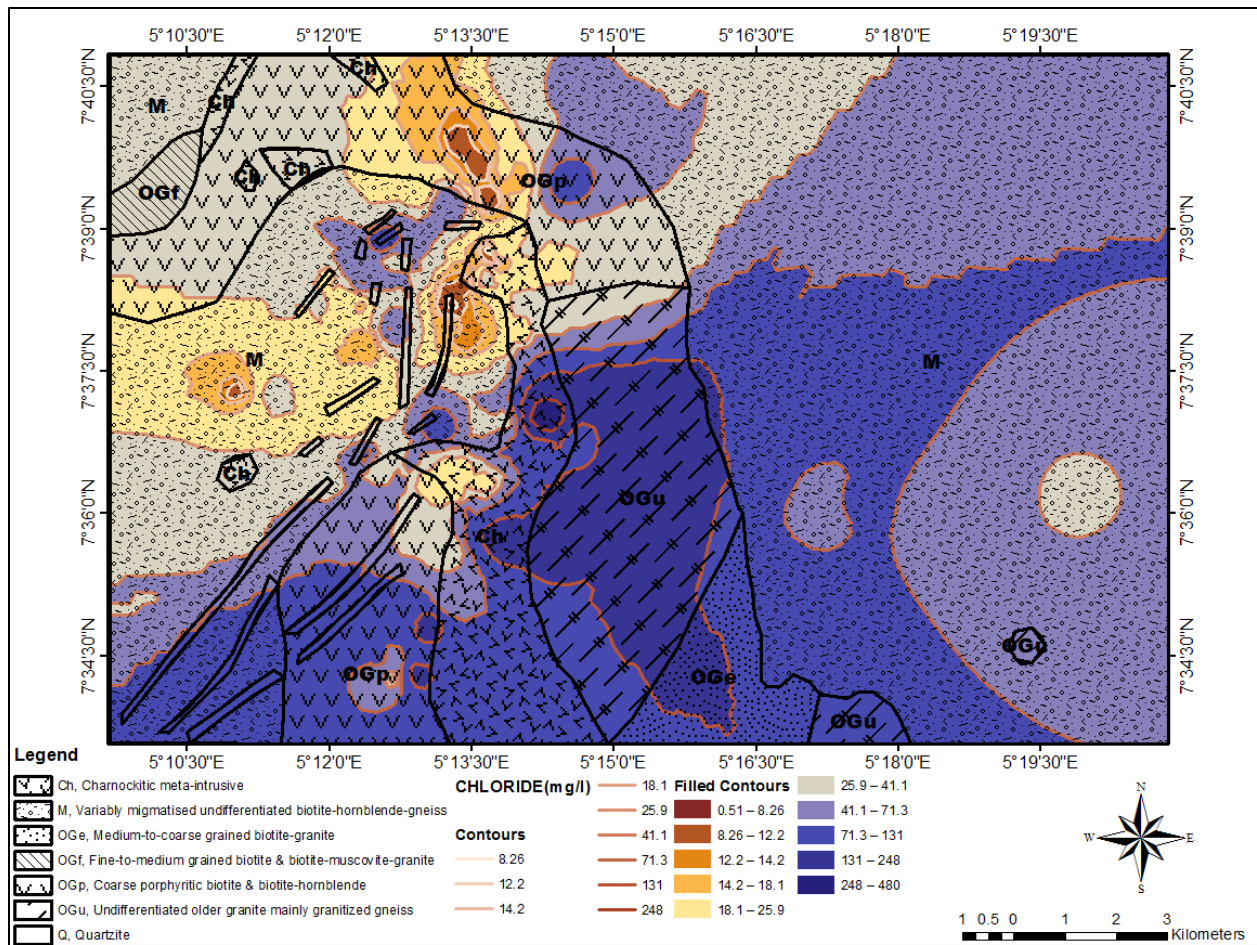
Figure 5.47: Chloride map
