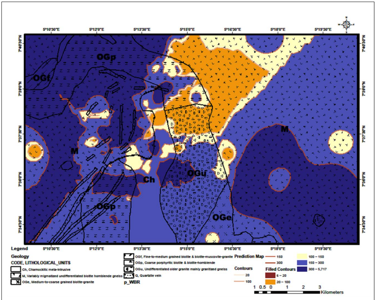
Figure 5.16: Weathered Basement Resistivity Classification Map
