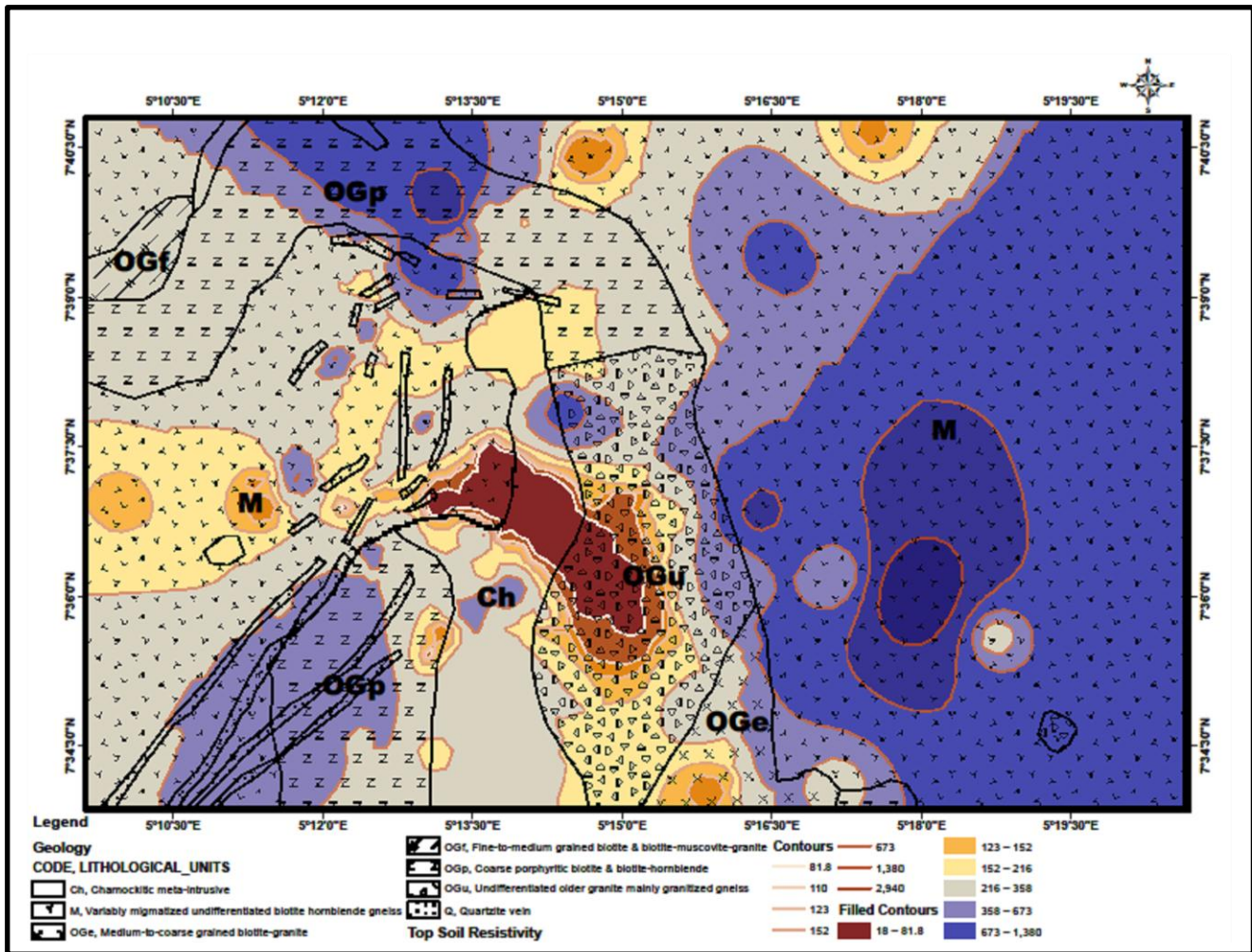
Figure 5.8: Topsoil Resistivity map
