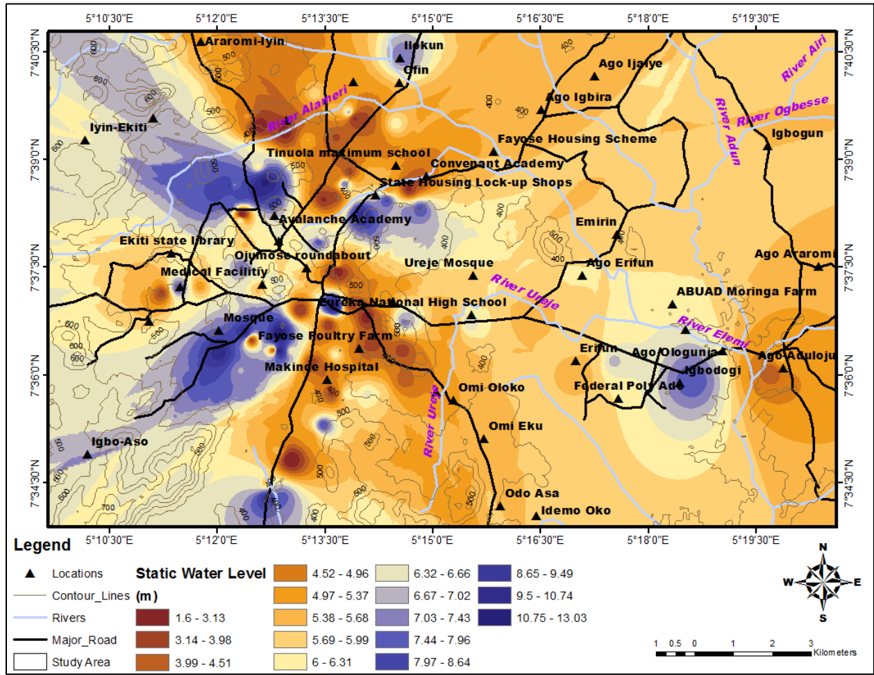
Figure 5.36: Static water level map
