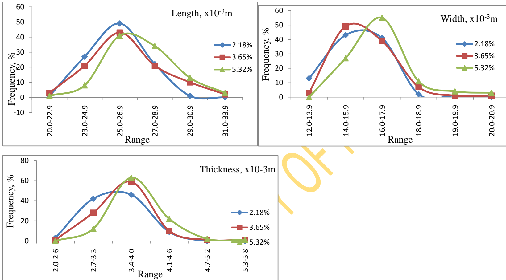
Fig. 4.3: Normal Distribution for Irvingia gabonensis kernel dimensions at different moisture contents
