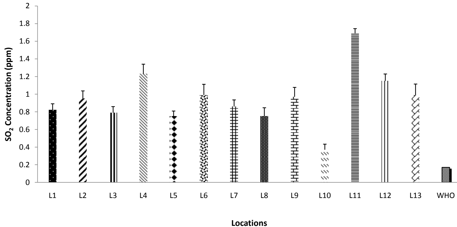
Figure 4.4: Comparison of weekly mean SO 2 concentration with WHO guideline limit for all the thirteen locations in the afternoon
