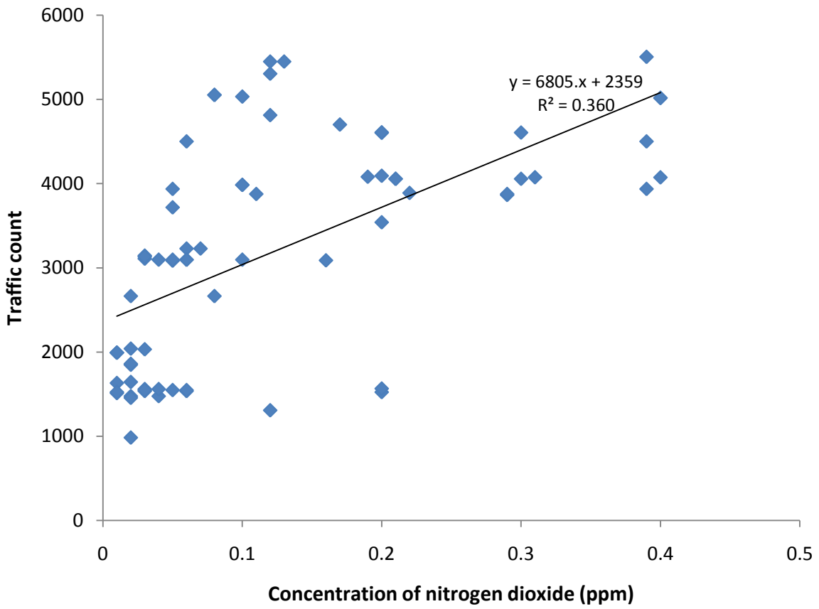
Figure 4.17: Relationship between traffic count and concentration of nitrogendioxide
