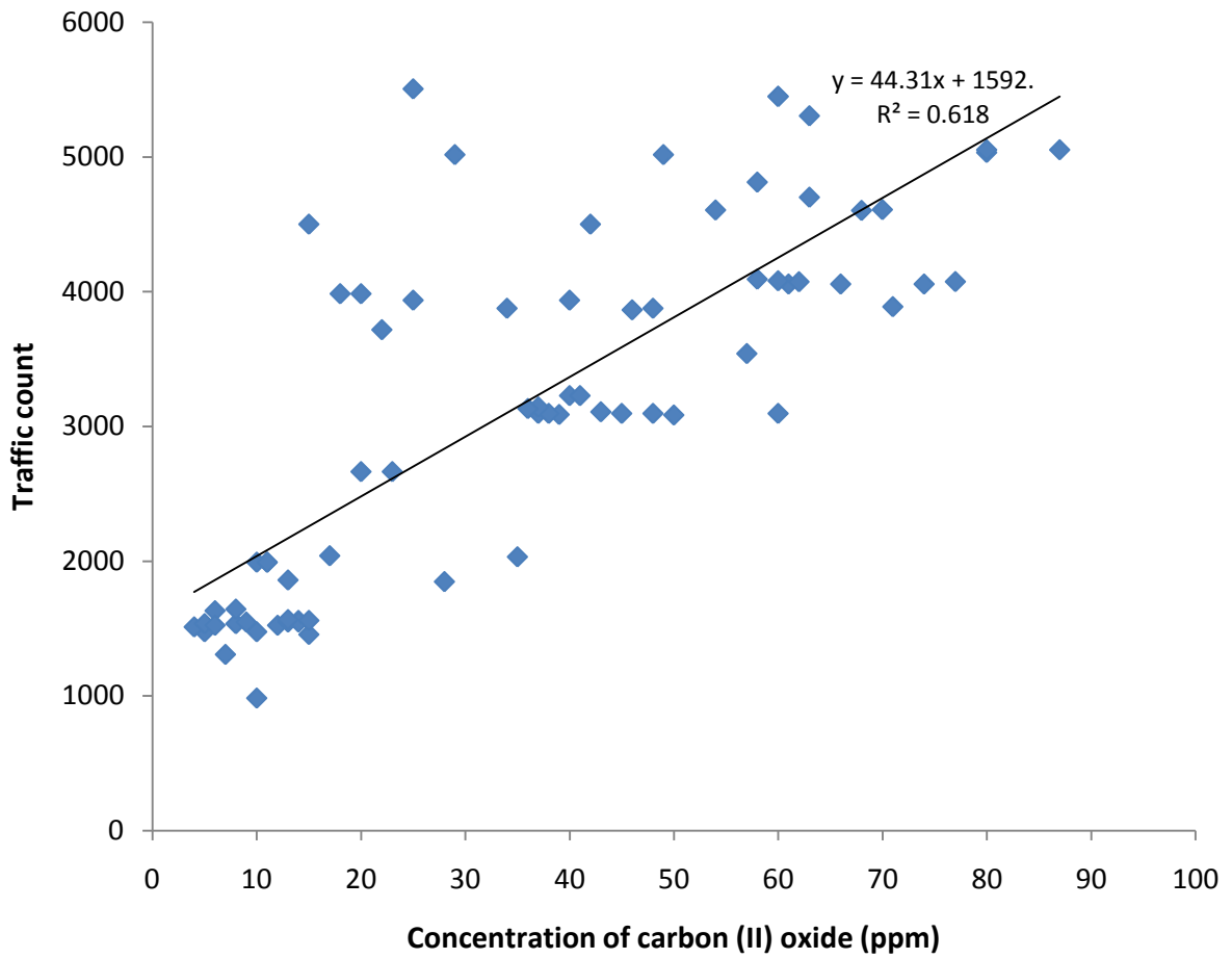
Figure 4.18: Relationship between traffic count and concentration of carbon (II) oxide
