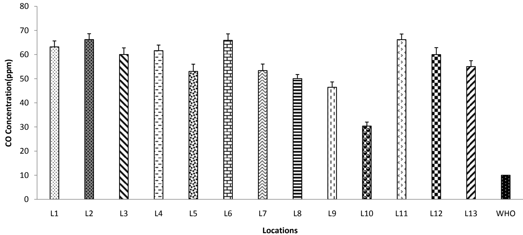
Figure 4.8: Comparison of weekly mean CO concentration with WHO guideline limit at all the thirteen locations in the evening
